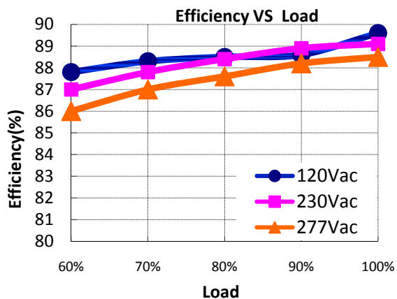
X6-060Y057( I_o=1.05A )
