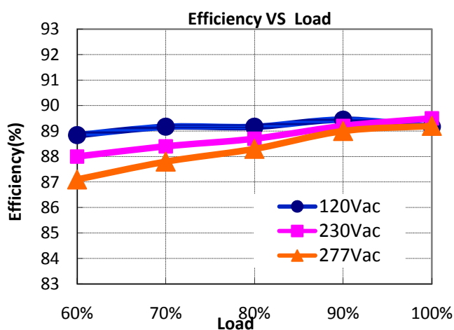
X6-060Y086( I_o=0.70A )
