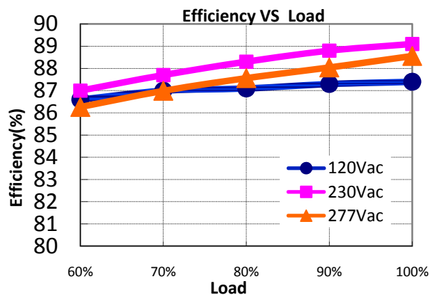
X6-060Y057( I_o=1.05A )
