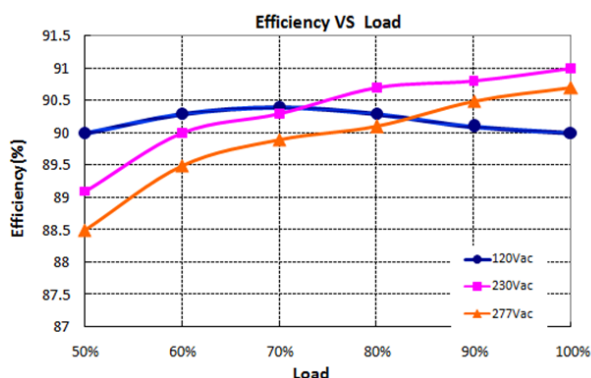
X6-060Y120( I_o=0.50A )
