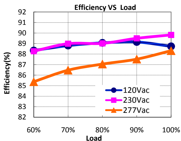
X6-060Y120( I_o=0.50A )
